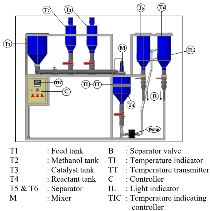
Figure 1. Biodiesel production using induction heating technology instrumentation
