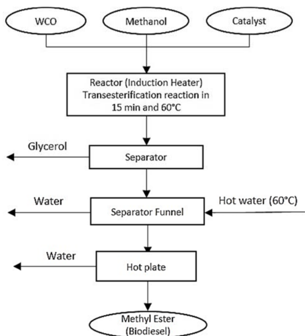
Figure 2. Flowchart for producing biodiesel with induction heating
